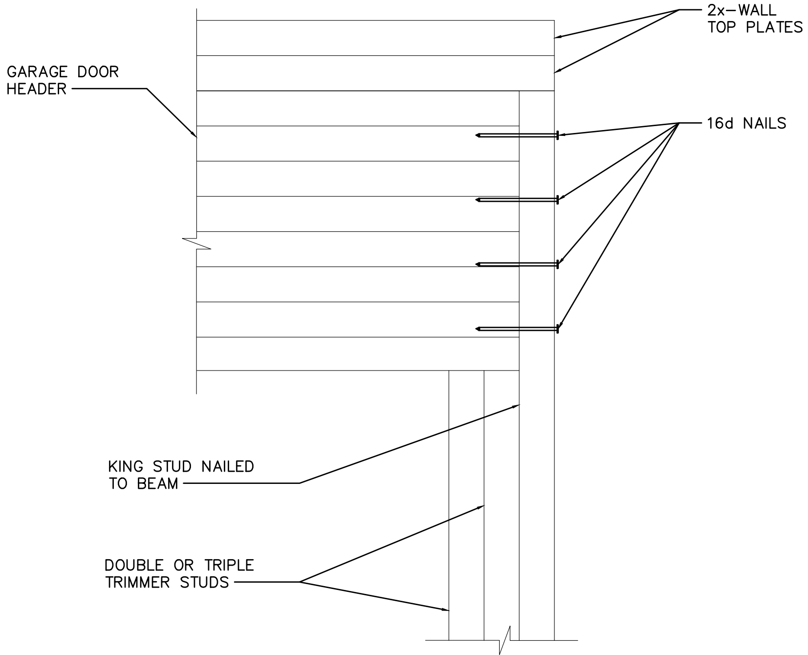
GH-1 GRG DR HEADER TO END WALL KING STUD NAILED TO BEAM
